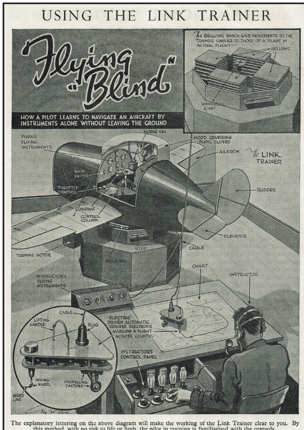
A Link Trainer depicted in a WW2 magazine article from Australia. Author's collection.
